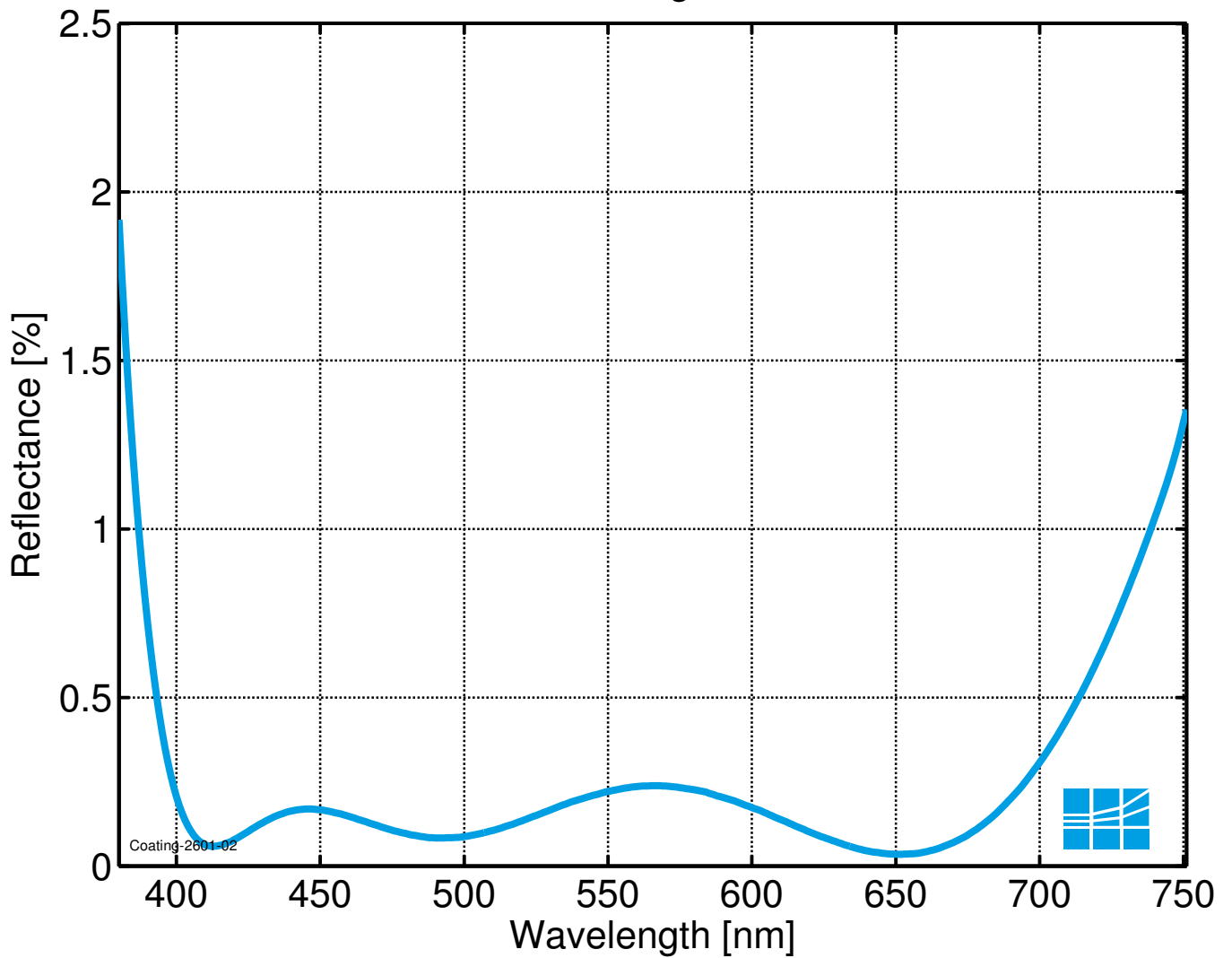
Coating-26
