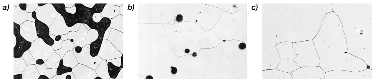
Fig. 3: Ice core sample images from different depths. All scans are obtained using the Large Area Scan Microscope. The ice core image from 60 m depth (a) shows grain boundaries and pores. These inclusions become rarer and smaller with depth (b; 615 m depth). Finally, at a depth of 1035 m almost all gas inclusions have transformed into air hydrates.
