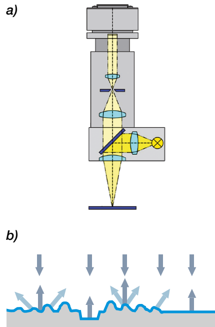
Fig. 4: Scheme of the Large Area Scan Microscope (a) and optical scheme of bright-field illumination (b) The light directed at the sample is reflected by surfaces parallel to the sensor. Light reflected from structures areas and edges is reflected away from the sensor and appear dark.
