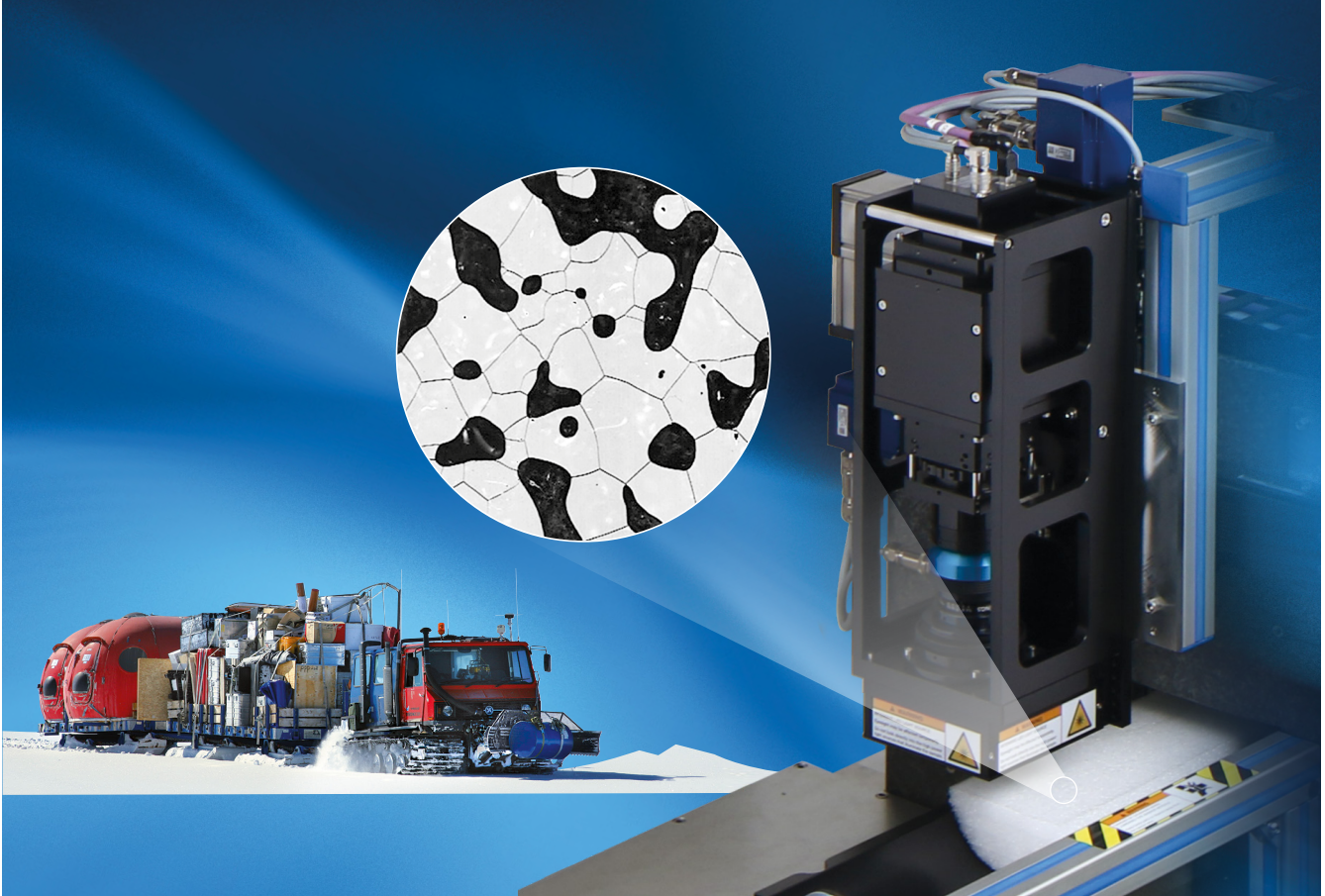
Fig. 1: Large Area Scan Microscope for the analysis of microstructure of polar ice cores. (Photo: Lars Berg Larsen, NEEM ice core project)
